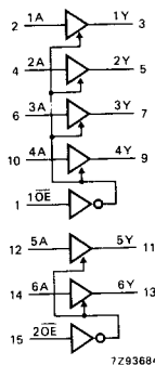
Fig. 2 Logic symbol.
