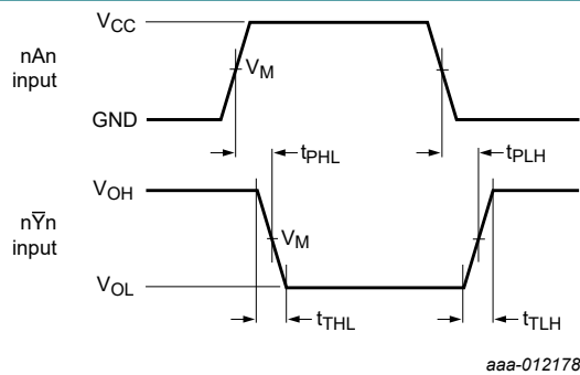
Fig. 7. Propagation delay input ( nA_n ) to output ( n\bar{Y}_n ) and transition time output ( n\bar{Y}_n )
