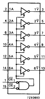
Fig. 4 Functional diagram.
