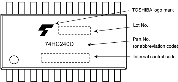
74HC240D
