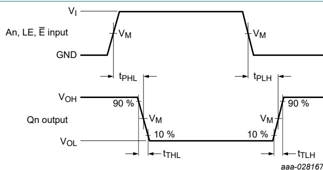
Fig. 7. The inputs (An, LE, \bar{E} ) to output (Qn) propagation delays and the output transition times
