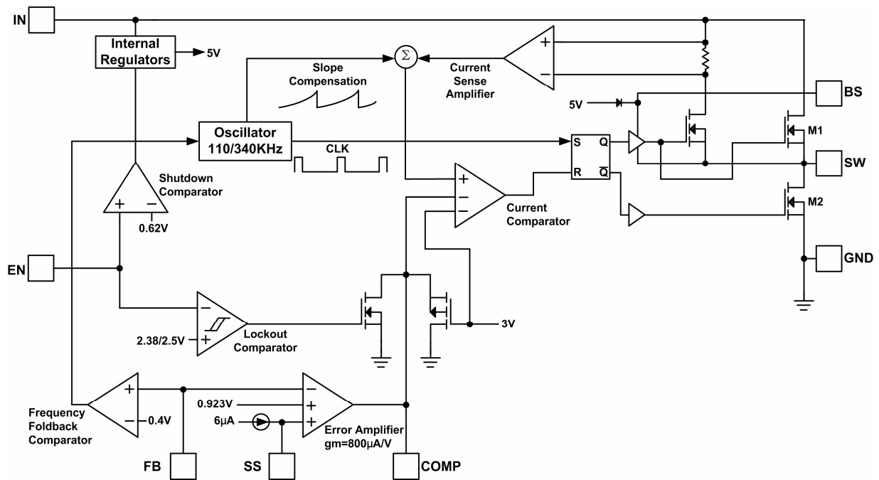
Figure 3.Functional Block Diagram
